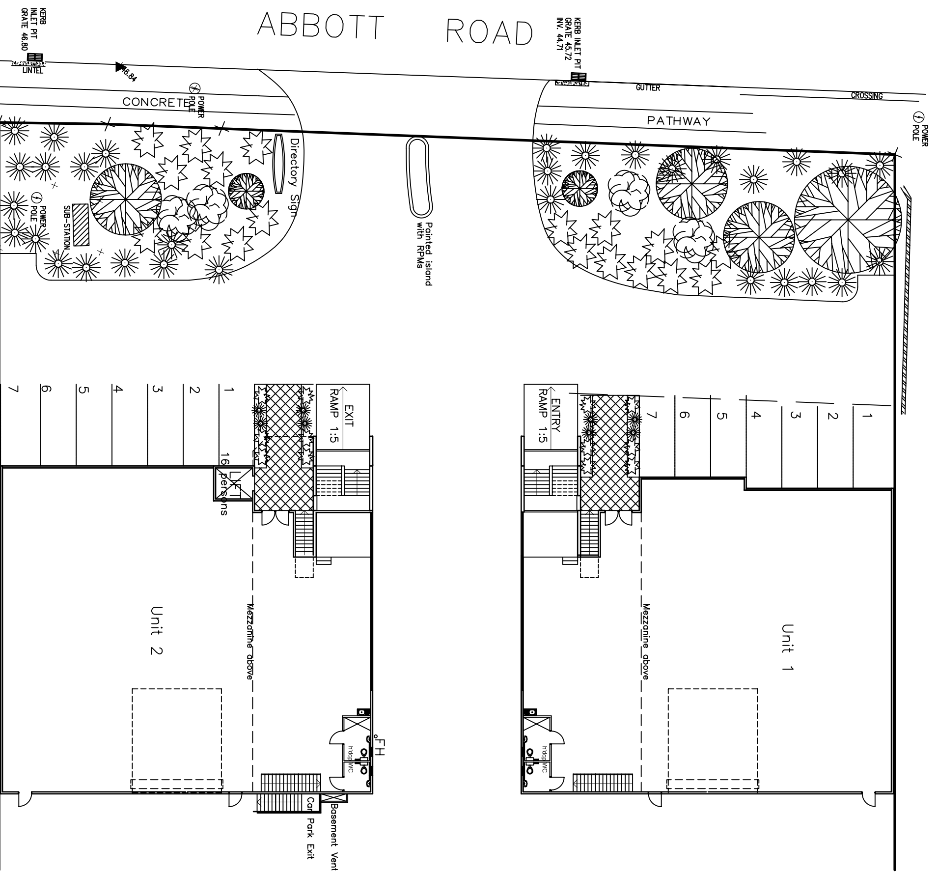
GROUND FLOOR PLANS
